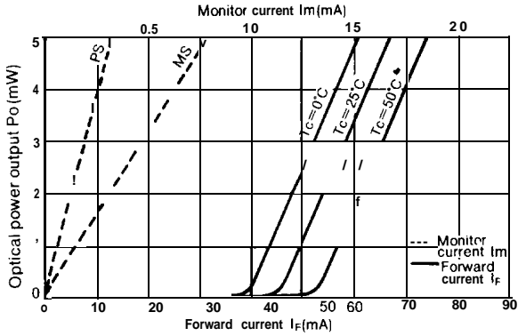
Fig. 93-2 Optical Power Output vs. Forward Current and Monitor Current
