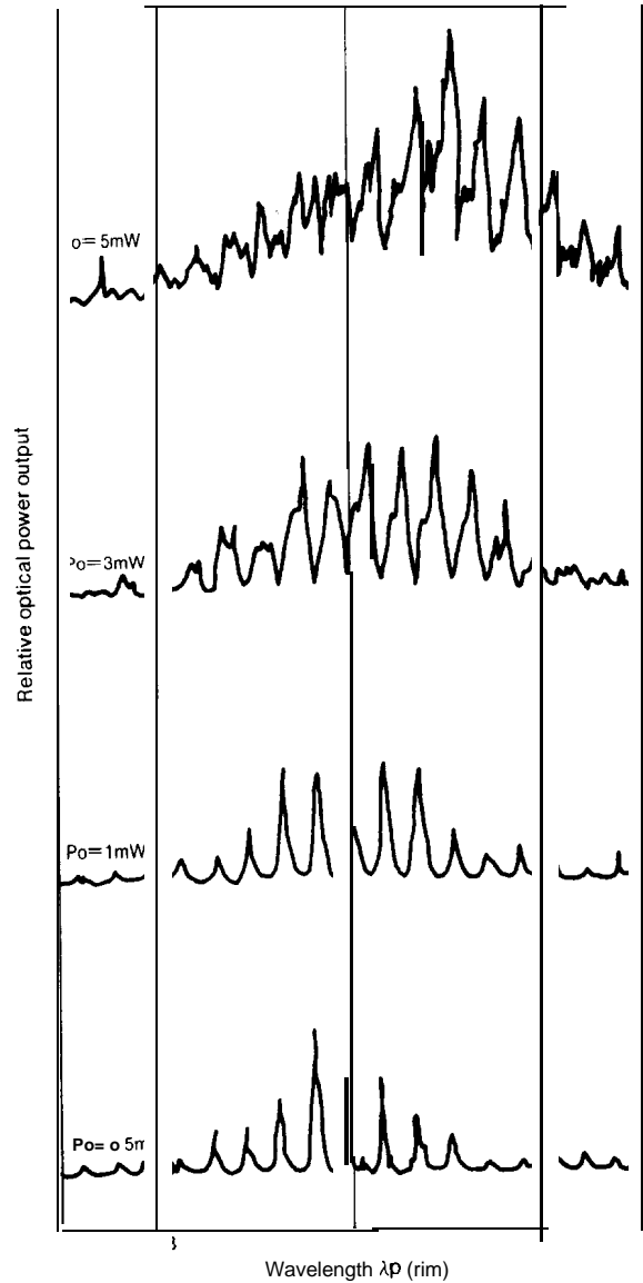
Fig. 93-5 Optical Power Output Dependence of Wavelength
