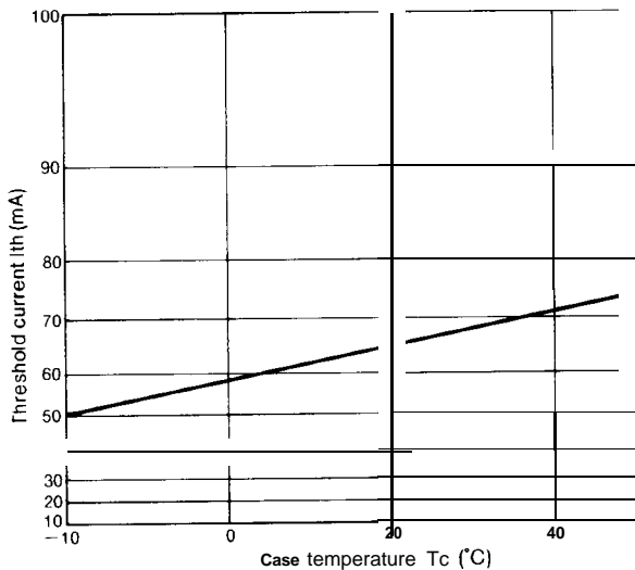
Fig. 93-3 Threshold Current vs. Temperature
