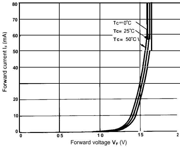
Fig. 93-1 Forward Current vs. Forward Voltage
