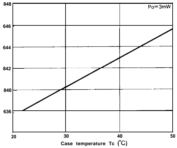
Fig. 93-4 Wavelength vs. Temperature
